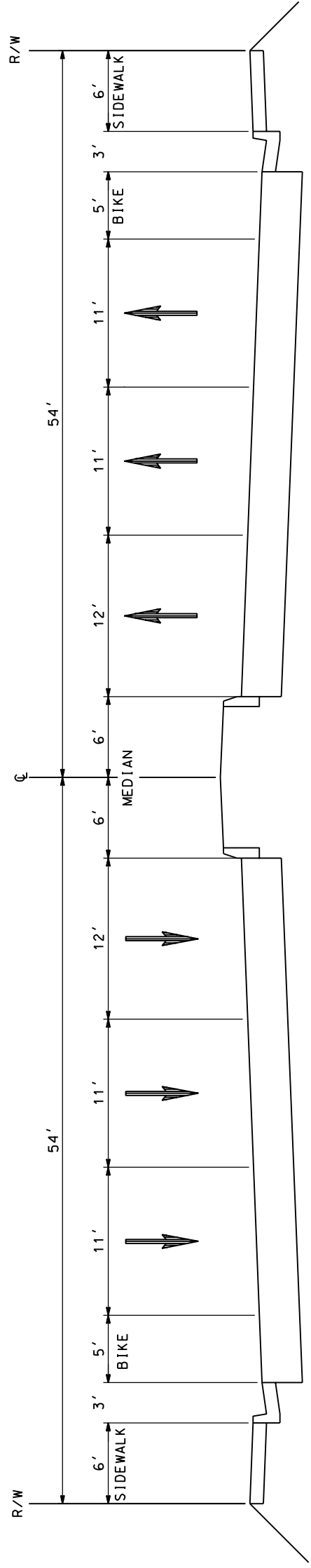
TYPICAL SECTION HAZEL AVENUE
